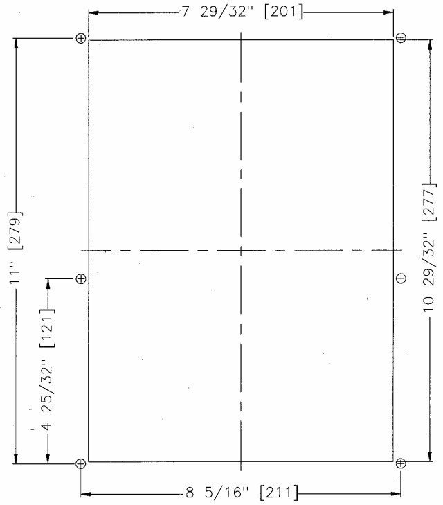
Cut-out Dimensions
